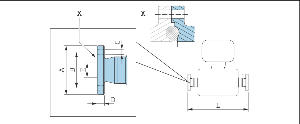
25 Detail X: Asymmetrical process connection; the part shown in gray is provided by the supplier.
