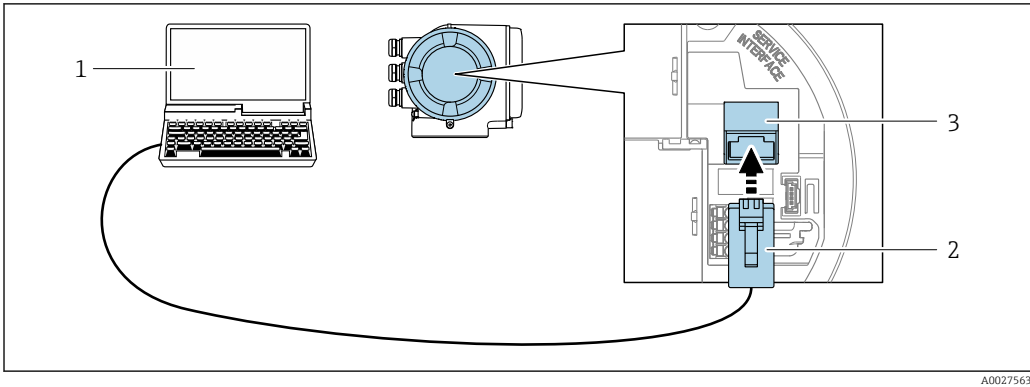
36 Connection via service interface (CDI-RJ45)
