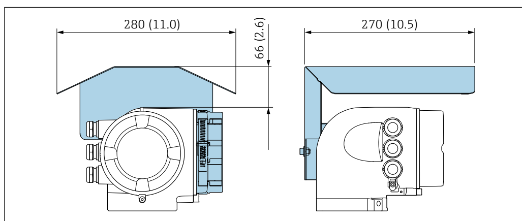
24 Weather protection cover for Proline 500
